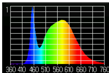
Spectrum of light 5000K
