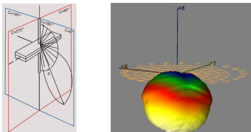
Luminaire light distribution of the 3D
